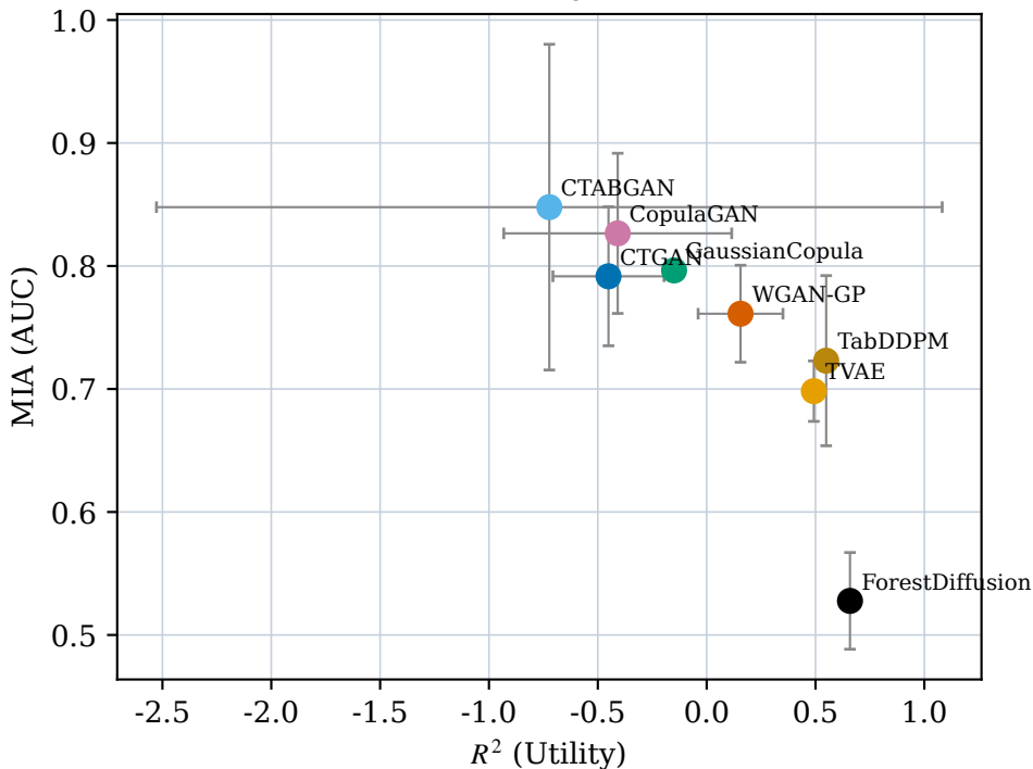
Concrete: R^2 (Utility) vs MIA (AUC)
